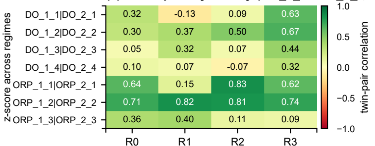
(c) Twin-pool symmetry (DO_1_* ↔ DO_2_*, ORP)
